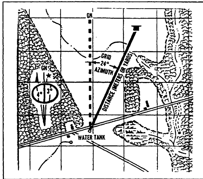
Figure 1-13. Polar coordinates used to designate position on map
